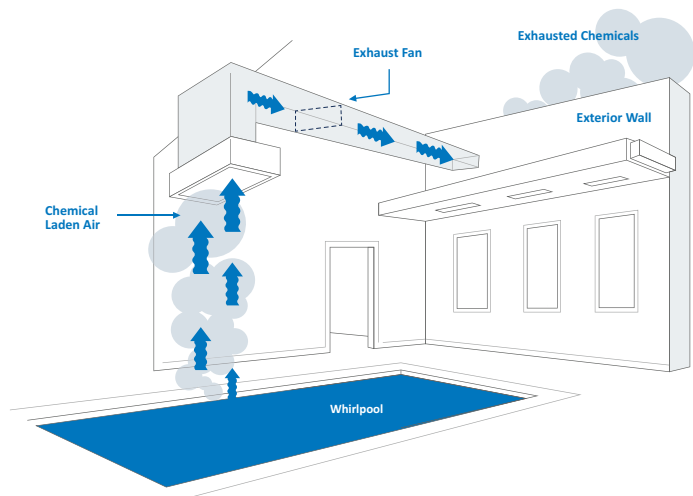
FIGURE 3: EXHAUST AIR
