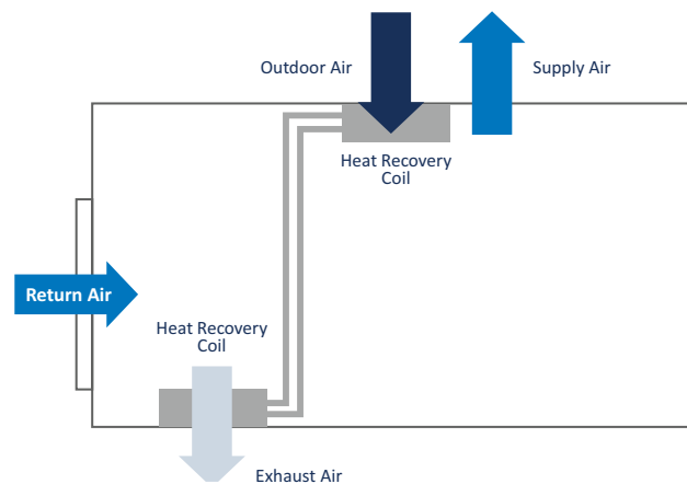
FIGURE 11: PACKAGED HEAT RECOVERY
