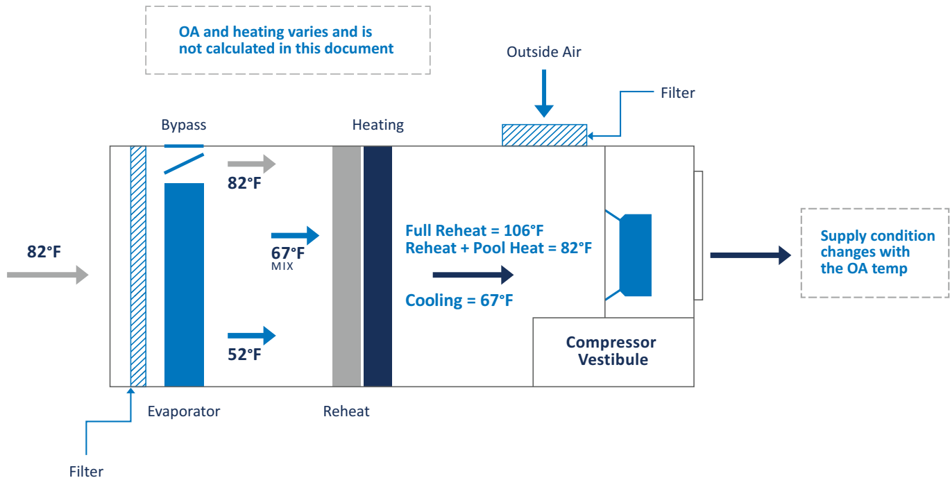
FIGURE 20: REFRIGERATION-BASED DEHUMIDIFIERS
