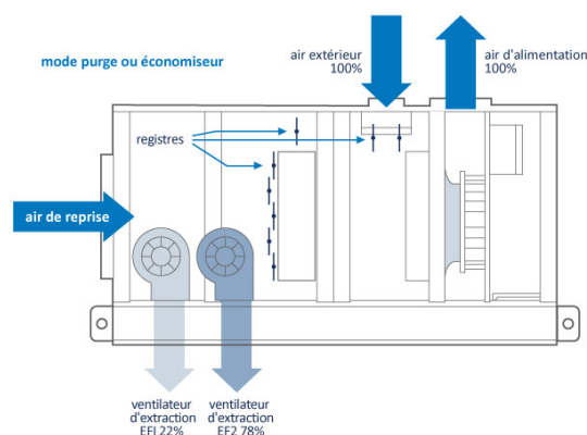
FIGURE 16 : MODE PURGE-ECONOMIZER
