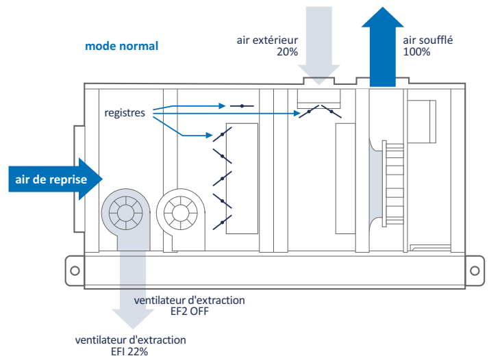
FIGURE I4 : MODE NORMAL
