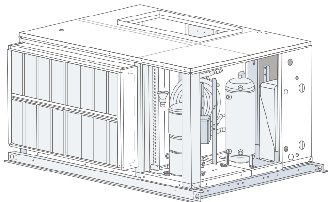
FIGURE 12 : ARMOIRE SLB
